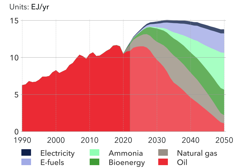
World maritime subsector energy demand by carrier
