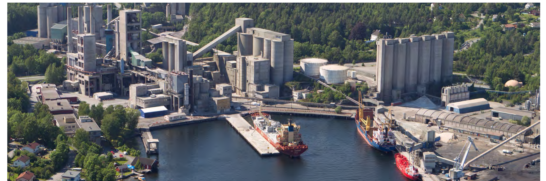
Brevik CCS - the world's first CO 2 -capture facility at a cement plant. Image courtesy, Heidelberg Cement
