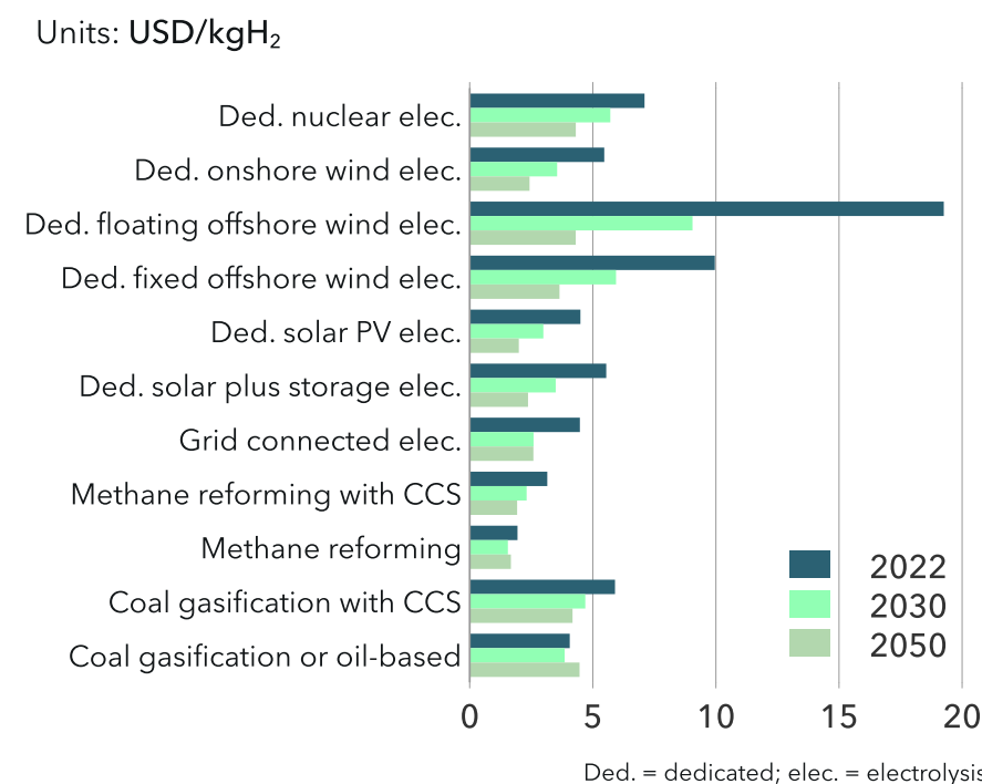
FIGURE 8.2.5 Latin America levelized cost of hydrogen production
