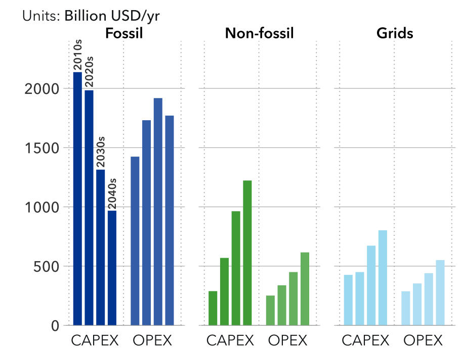
FIGURE 5.2 World energy CAPEX and OPEX, 10-year average
